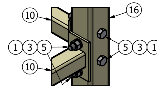
DETAIL D
