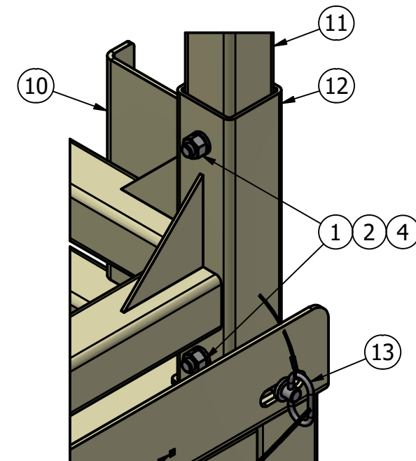
ANCHOR POINT FOR PIN LANYARD DETAIL C
