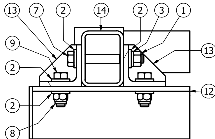
DETAIL F
