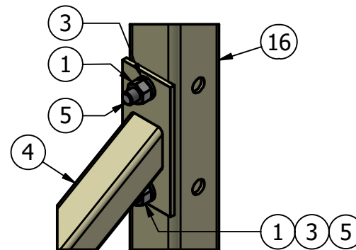
DETAIL C
