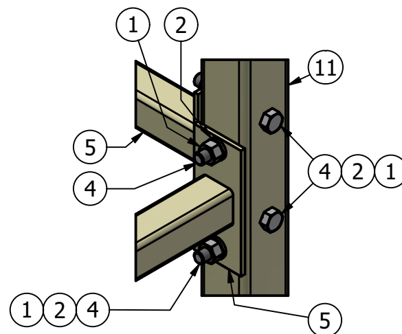
DETAIL B
