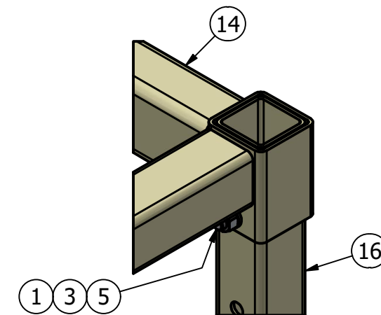
DETAIL B
