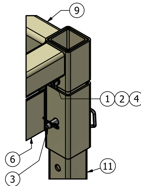
DETAIL A
